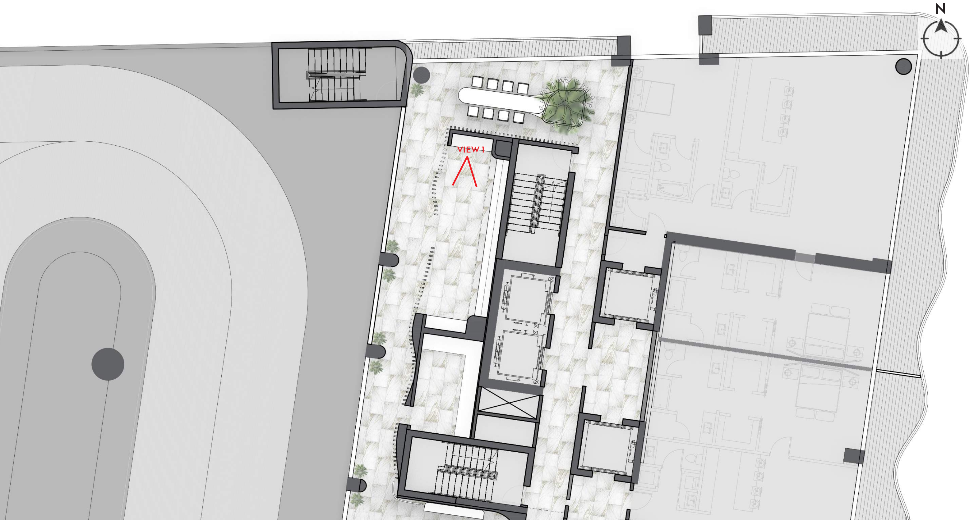
MAIL AND PACKAGE ROOM PLAN
